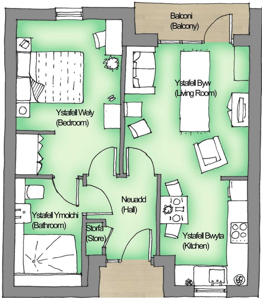
Cynllun o fflat nodweddiadol 50sqm 2 1Gwely 2Berson (Typical 1Bed 2Person flat layout 50sqm 2 )
